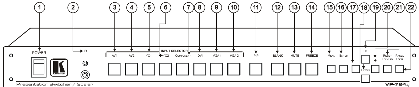
Figure 5: VP-724xl Presentation Switcher / Scaler Front Panel
