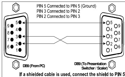
Figure 8: Connecting the PC
