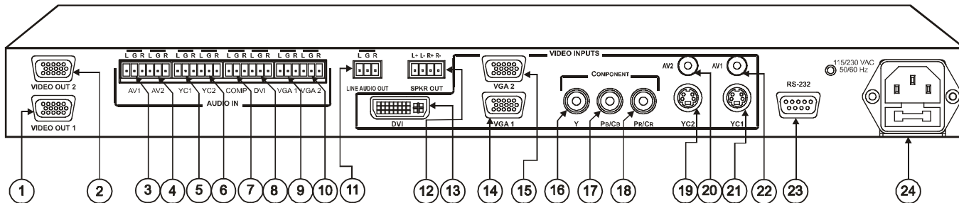
Figure 6: VP-724xl Presentation Switcher / Scaler Rear Panel
