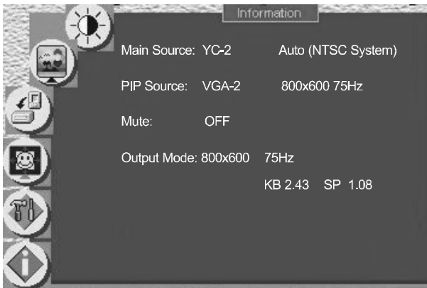
Figure 44: Information Screen
